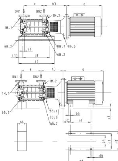
Fig. 6: Multitec E dimensions
