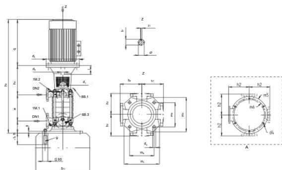
Fig. 8: Dimensions of Multitec V / Multitec-RO
