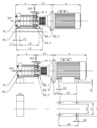
Fig. 7: Multitec F dimensions
