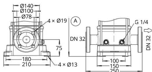
Fig. 20: Connections of Movitec VCF
