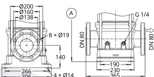
Fig. 53: Connections of Movitec VCF (DN 80)
