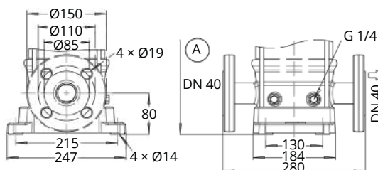
Fig. 30: Connections of Movitec VF, VSF
