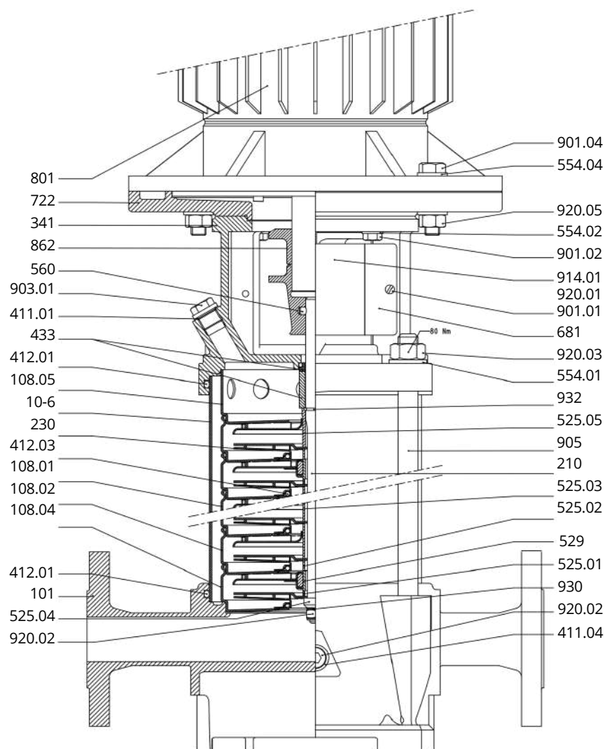
Fig. 83: General assembly drawing Movitec LHS
