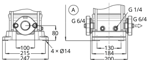
Fig. 27: Connections of Movitec V, VS
