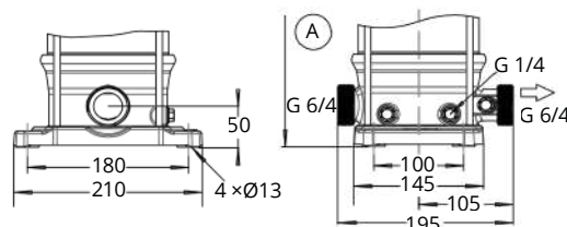
Fig. 20: Connections of Movitec VCF
