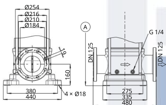
Fig. 68: Connections of Movitec VF, VSF, VCF (PN 16)
