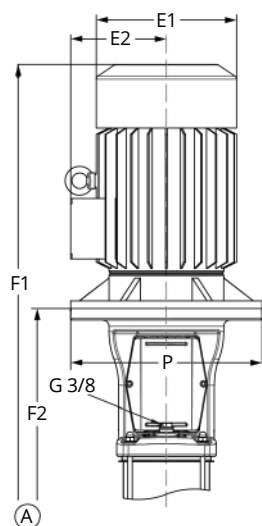
Dimensions of Movitec V(S), V(S)V, V(S)T, V(C/S)F
