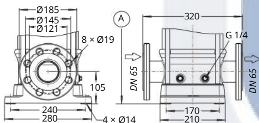
Fig. 44: Connections of Movitec VF, VSF
