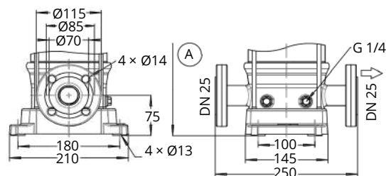
Fig. 7: Connections of Movitec VF, VSF
