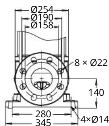
Fig. 63: Connections of Movitec VCF (PN 25, PN 40)
