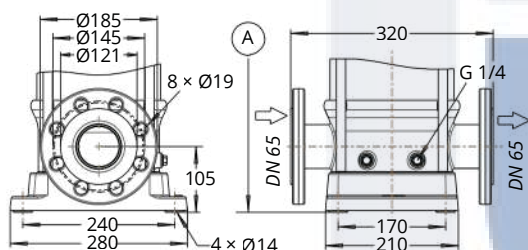
Fig. 42: Connections of Movitec VF, VSF
