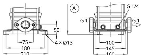
Fig. 4: Connections of Movitec V, VS
