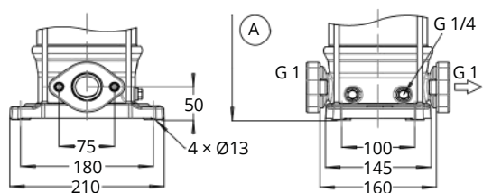
Fig. 10: Connections of Movitec V, VS
