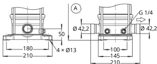
Fig. 17: Connections of Movitec VV, VSV
