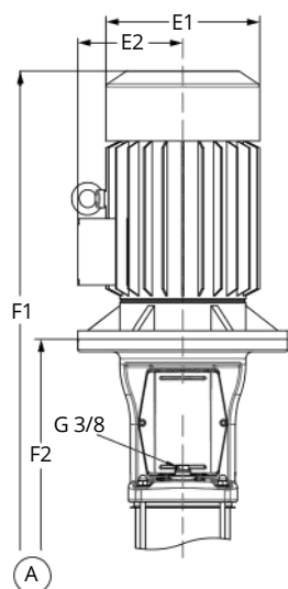
Dimensions of Movitec V(S), V(S)V, V(S)T, V(C/S)F
