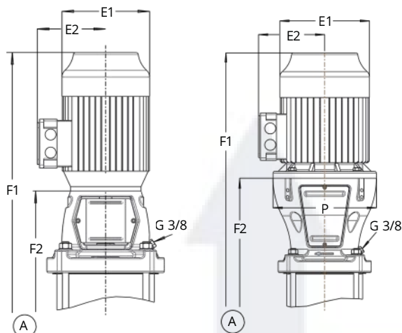
Dimensions of Movitec V(C/S)F
