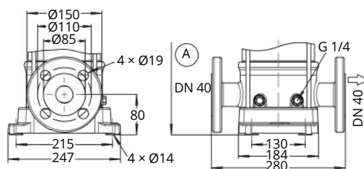
Fig. 30: Connections of Movitec VF, VSF
