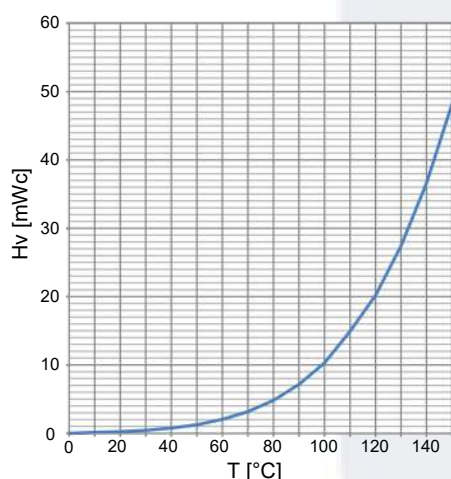
Fig. 2: Vaporisation pressure (Hv) diagram for water
