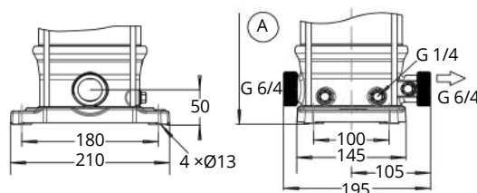
Fig. 14: Connections of Movitec VCF
