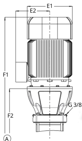
Dimensionsof Movitec V(C/S)F
