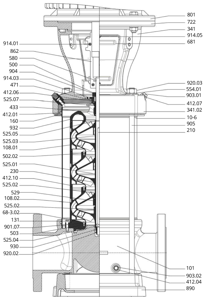
Fig. 82: General assembly drawing Movitec125B
