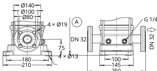
Fig. 19: Connections of Movitec VF, VSF
