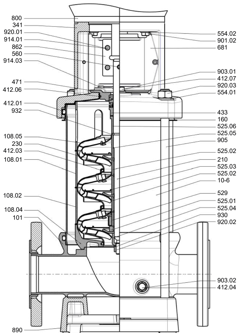
Fig. 79: General assembly drawing Movitec 25B
