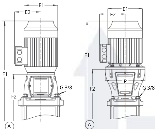
Dimensions of Movitec V(C/S)F
